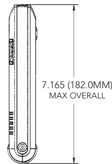
MVP-8400 (Right Side)
