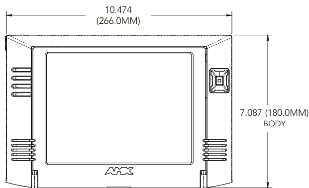
MVP-8400 (Front View)
