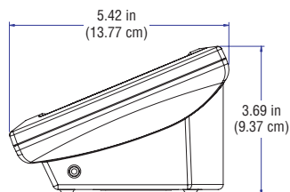
ST-1550C Touchpanel Right Side View
