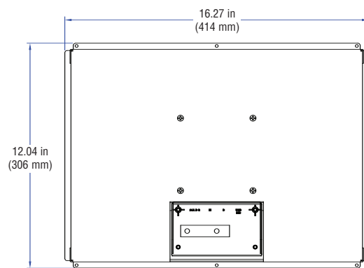
V15-WALL Wall Mount Model – Front View (w/Bezel), Side & Rear Views (w/o Bezel)
