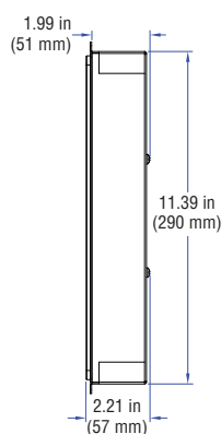
V15-WALL Wall Mount Model – Front View (w/Bezel), Side & Rear Views (w/o Bezel)
