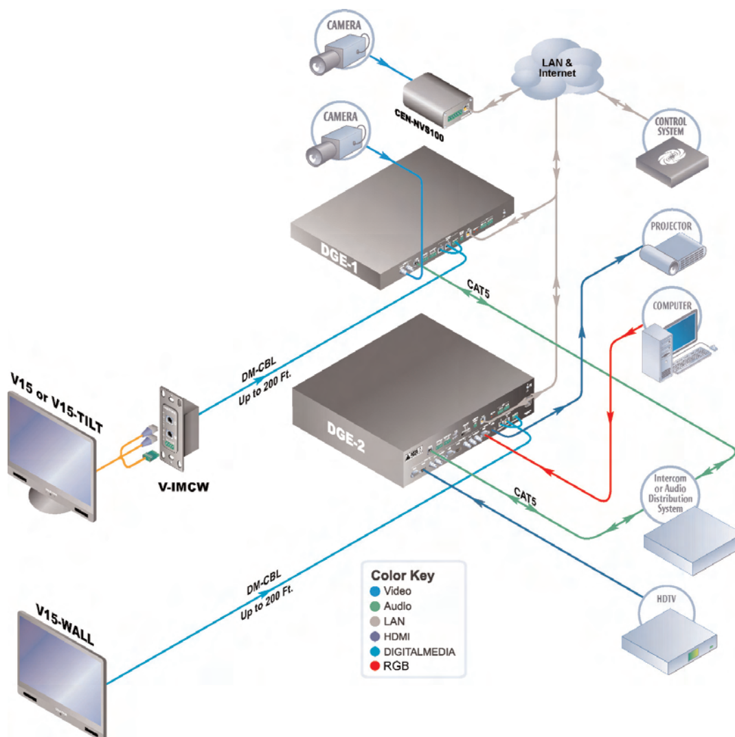
Typical Application
