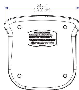
Docking Station - Bottom View
