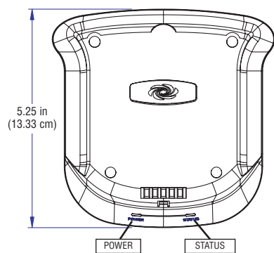
Docking Station - Top View
