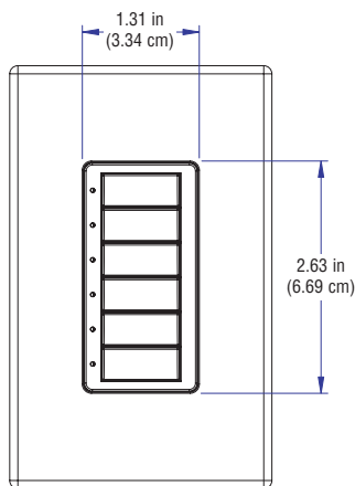
C2N-CBD – Front View (shown with faceplate, not included)
