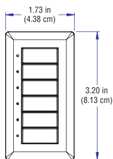
C2N-CBF – Front View (shown without spring clamp)
