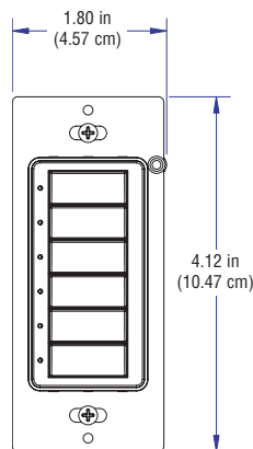
C2N-CBD – Front View
