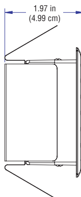
C2N-CBF – Side View
