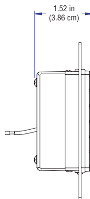
C2N-CBD – Side View
